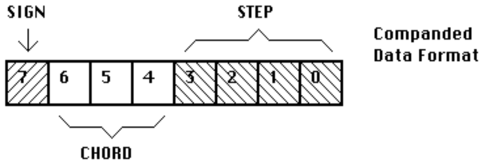
Figure 11 - Companded Data Format
